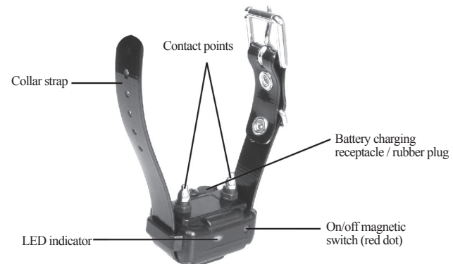
Receiver/Collar
