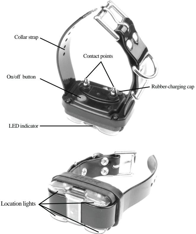
EDGE Receiver/Collar
